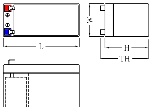
DIMENSIONS (치수)
