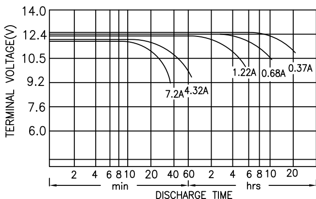
DISCHARGE CURVES (25 °C. 77 °F) (방전곡선)
